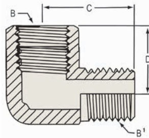
FULL PATTERN 90° STREET ELBOW- Extruded NPTF - Dryseal Ref. SAE 130239
