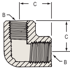
90° FEMALE PIPE ELBOW- Extruded NPTF - Dryseal Ref. SAE 130238
