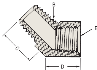
45° STREET ELBOW- Extruded NPTF - Dryseal Ref. SAE 130339
