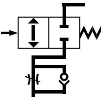
Speed control and blocker
