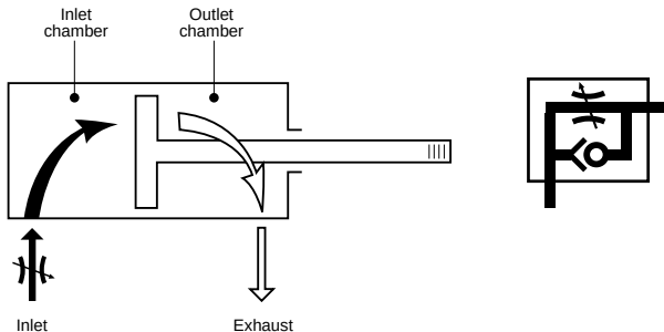
Flow regulation on the inlet port
