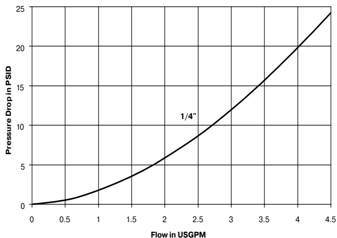
SM Series (1/4") Test Fluid: Oil - 200 SUS
