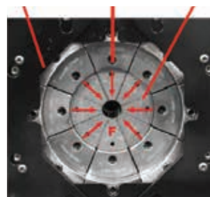
Fixed 6:00 die for easy positioning of fittings
