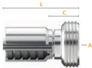
IHUM Fitting
